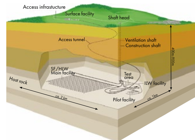
View of the Swiss concept for a SF/HLW/ILW repository in the Opalinus clay with inset of SF canister-emplacement tunnel and longitudinal section of emplacement tunnels for SF for the design option using low-pH shotcrete tunnel support. SF: Spent fuel; HLW: High-level waste; ILW: Intermediate-level waste.
