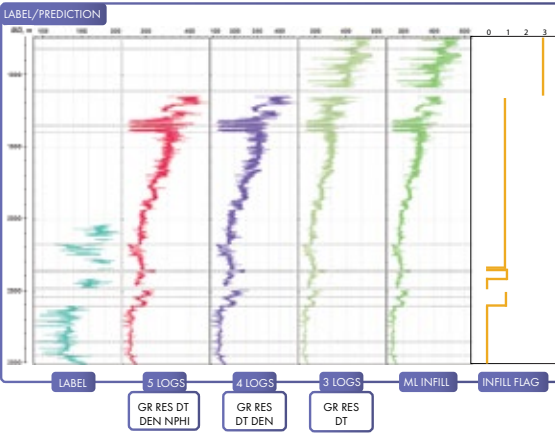
Figure 3: DTS machine learning model prediction and imputation, built using combinations of logs as features. The imputation priority goes from left to right on the, while the origin of the log prediction is shown by the ML-flag.
