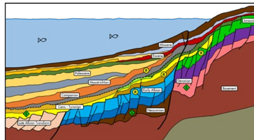
Figure 1: Geoseismic section sketch through the Keta Basin showing the tectonic architecture and the main hydrocarbon play elements.
